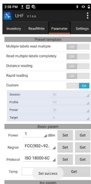
Figure 8-11 Query parameters
