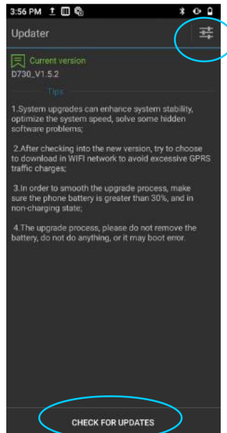
Figure 8-14 System upgrade
