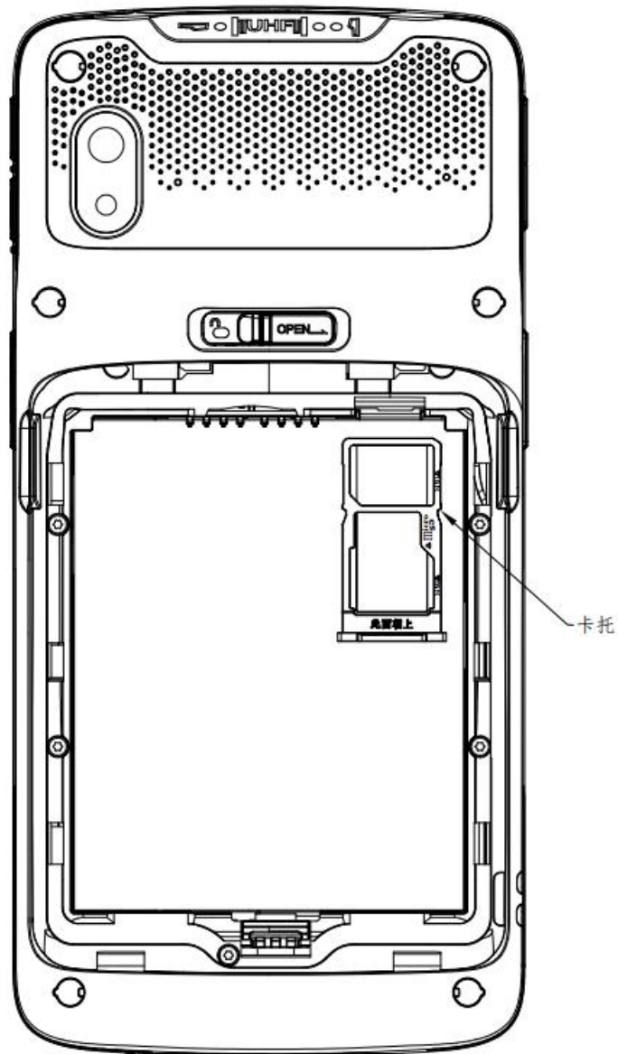
Figure 4-2 Insert the SD card
