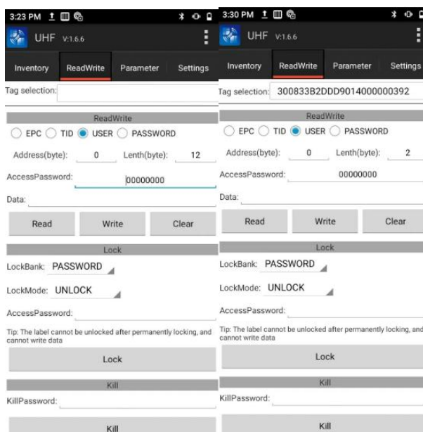
Figure 8-9 Read/write tag interface
