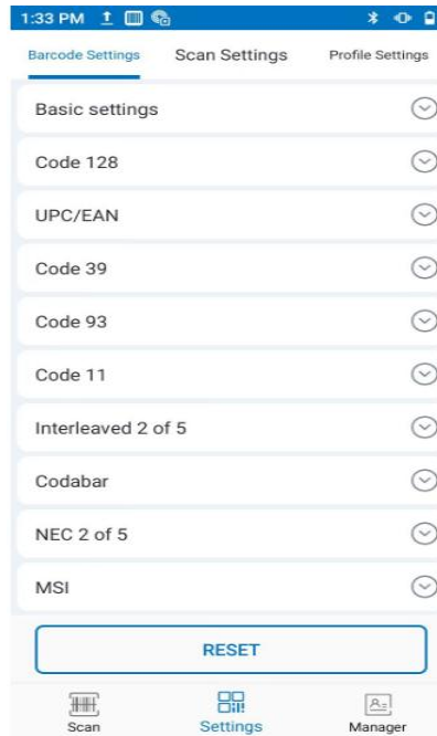
Figure 8-2 Barcode settings
