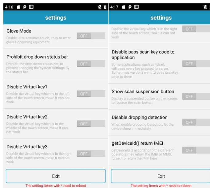
Figure 8-29 Feature settings
