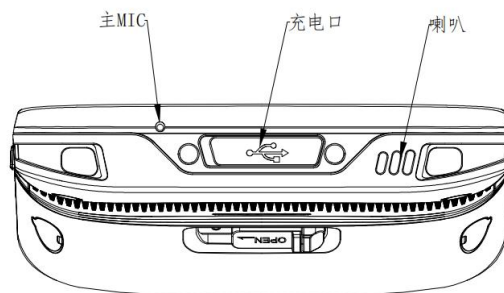
Figure 2-4 Rear view
