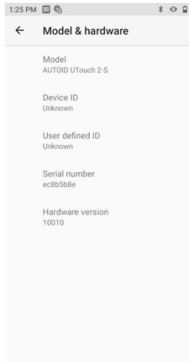
Figure 7-36 Model & Hardware
