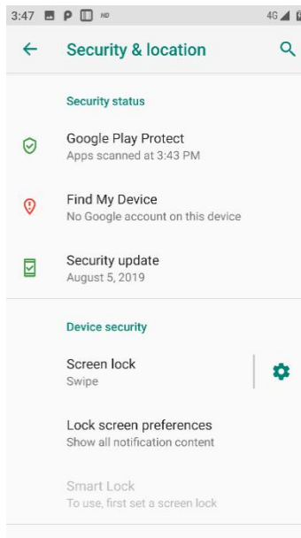
Figure 7-28 Security
