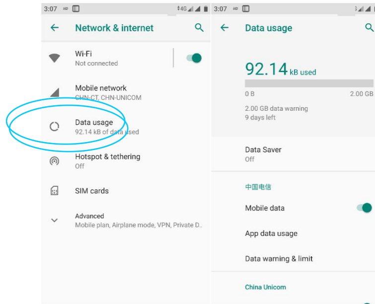
Figure 7-9 Traffic usage
