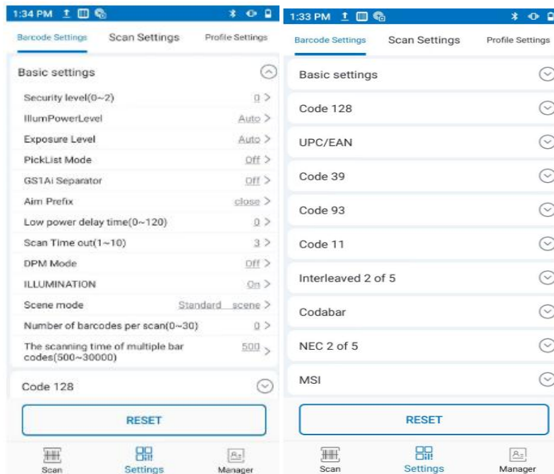
Figure 8-3 Basic settings
