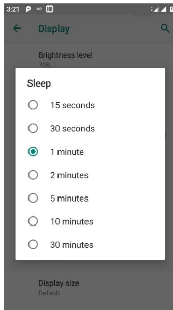
Figure 7-20 Sleep
