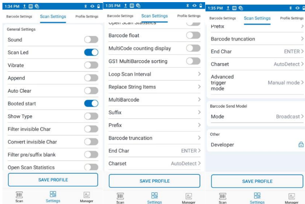
Figure 8-4 Application settings
