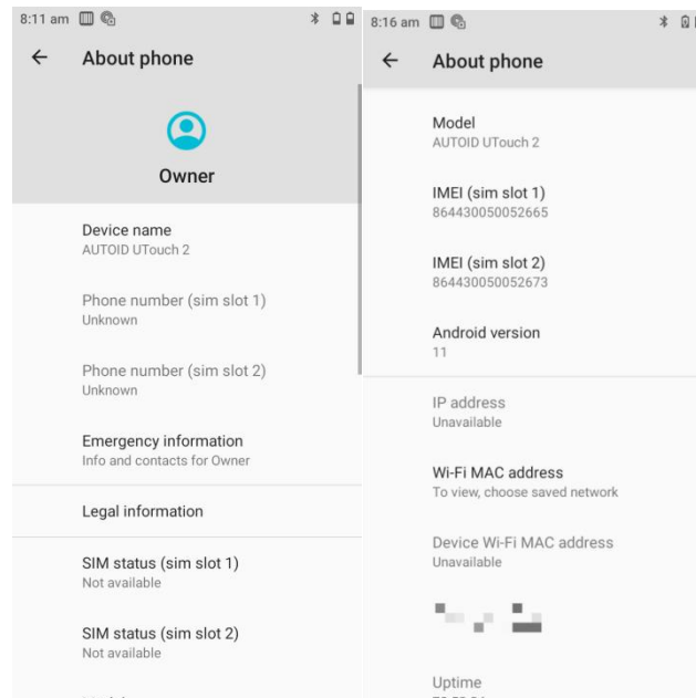
Figure 7-35 About phone
