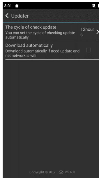
Figure 8-18 System upgrade
